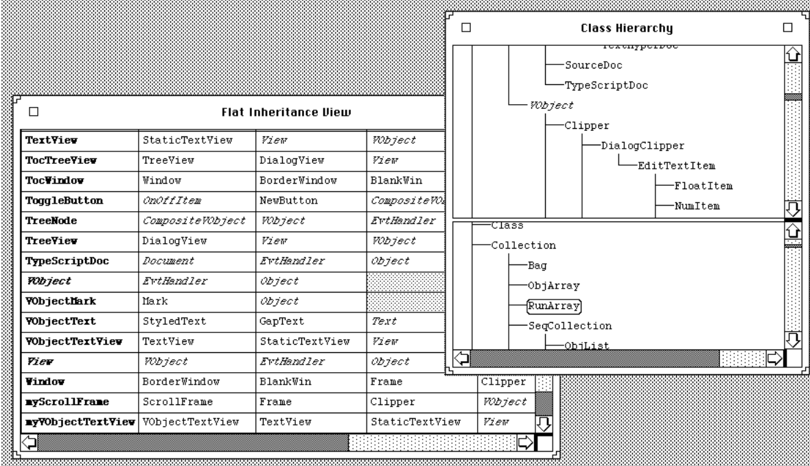
Figure 19. The Hierarchy Viewer.
