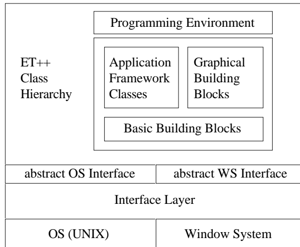
Figure 4. ET++ Architecture.
